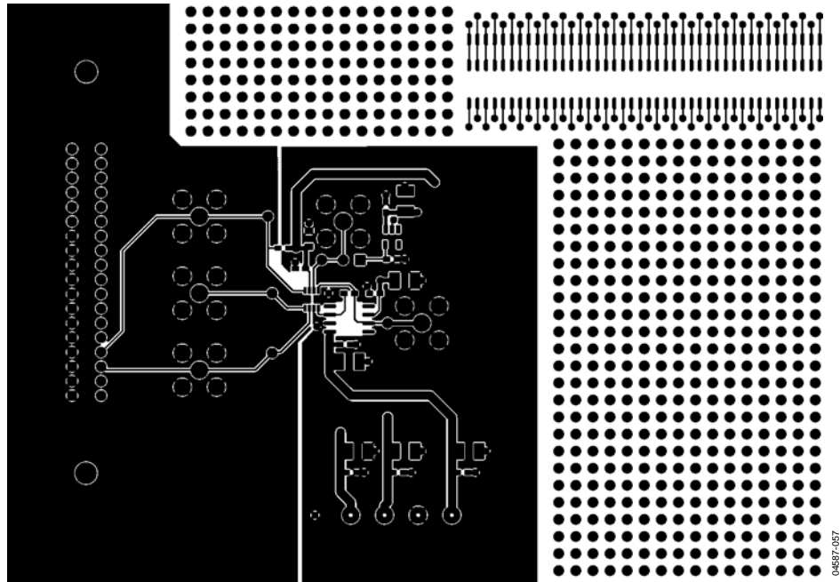
Figure 62. Component-Side Artwork
